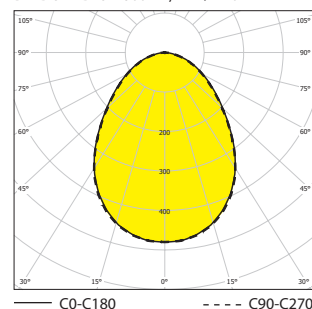
BALDO-LED-OP-800-4K, IP44/IP20
