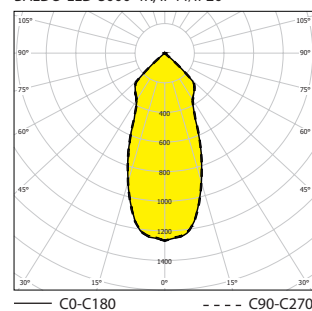
BALDO-LED-OP-800-4K, IP44/IP20
