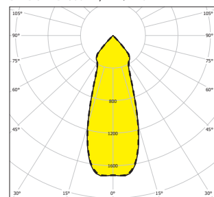
BALDO-LED-3000-4K, IP44/IP20
