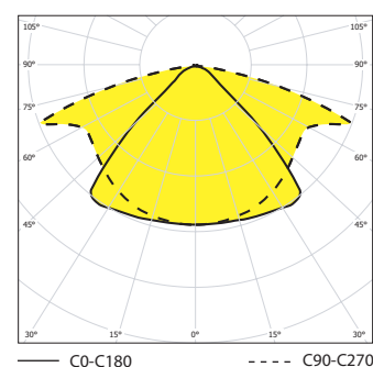
AQUARI 40-LED, 90° – IP 65
